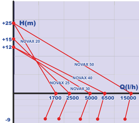
NOVAX 50 M
